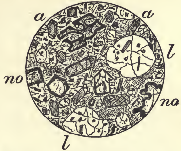
Fig. 37.—Nosean-Leucitite. Rieden, Eifel. \times 7 . a , Dark green pleochroic soda-augite, often zoned. l , Leucite, including small soda-augites and microscopic haüyenes. no , Nosean, with darkened and corroded borders. Hemicrystalline groundmass.
